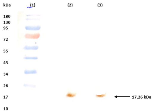
Gambar 3. Hasil uji Western blot.
